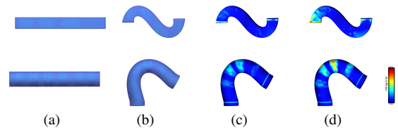
Fig. 10. Shape reconstruction for the deformed bar (top row) and cylinder (bottom row) shapes. (a) source mesh, (b) deformed mesh, (c) reconstructed mesh using cotangent weights (with error color coding), (d) reconstructed mesh using uniform weights (with error color coding).
